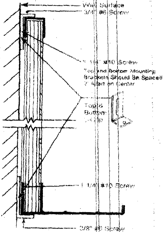
MARKER BOARDS STANDARD TRIM AND TRAY
