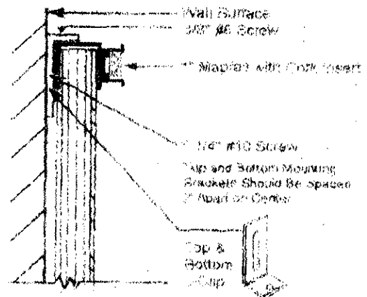
MARKER BOARDS STANDARD TRIM, BLADE TRAY, 1\"/>
