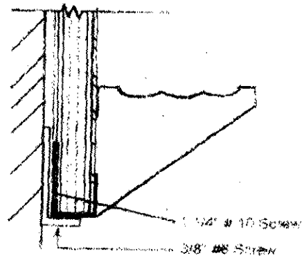
MARKER BOARDS STANDARD TRIM, BOX TRAY
